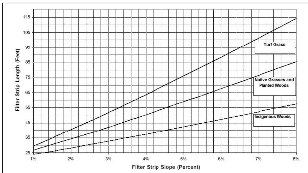
Figure 7: Loam, Silt-Loam Soils with HSG Group B Source: New Jersey Stormwater Best Management Practices Manual, February 2004
