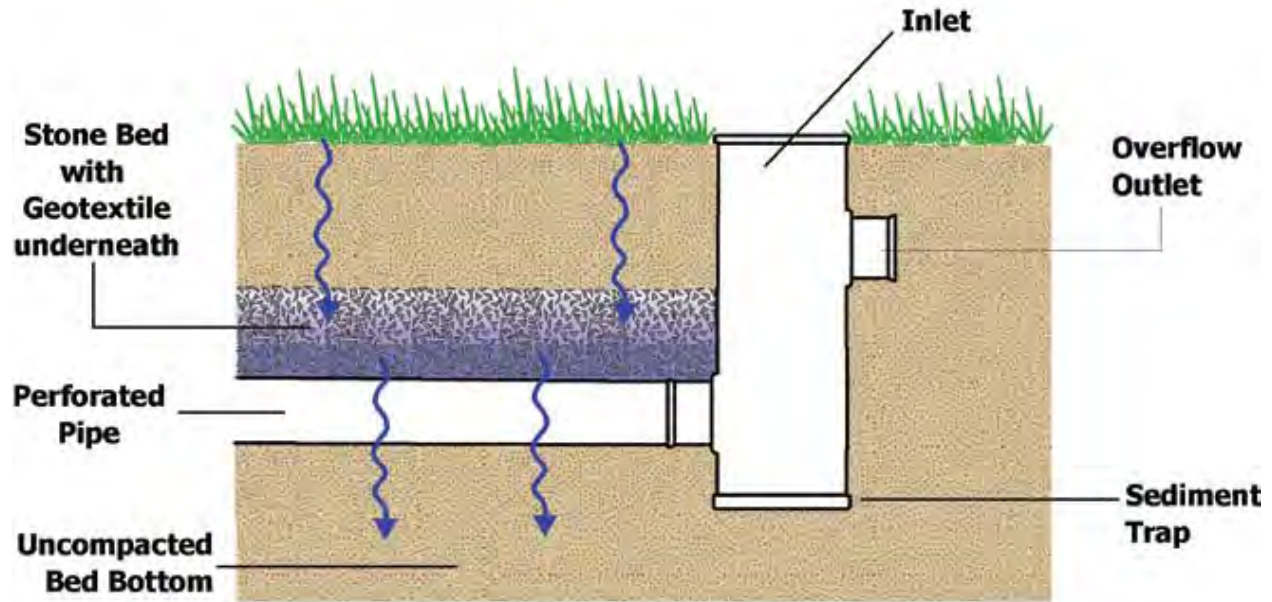
Figure 8 Schematic of subsurface infiltration bed cross section
