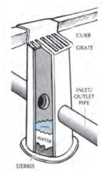
Figure 3: Sumped Catch Basin Source: City of Farmington Hills, MI
