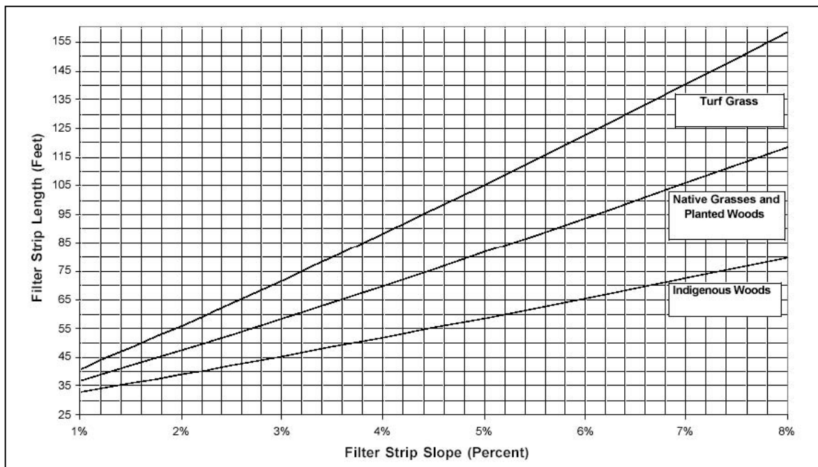
Figure 9: Clay Loam, Silty Clay or Clay Soils with HSG Group D Source: New Jersey Stormwater Best Management Practices Manual, February 2004
