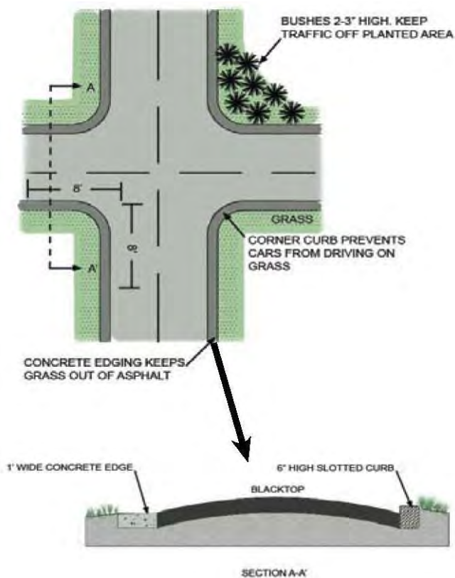
Curb cuts as a method of stormwater disconnection Source: Center for Watershed Protection, modified by Cahill Associates, 2008
