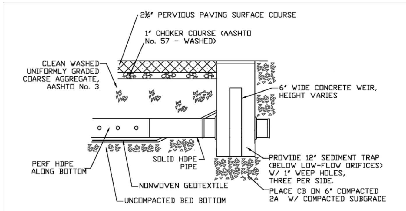
Figure 3: Example cross-section of porous asphalt system
