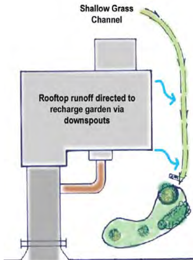
Figure 3 Single-family residential lot drainage schematic Claytor and Schueler, 1995 with modifications by Cahill Associates
