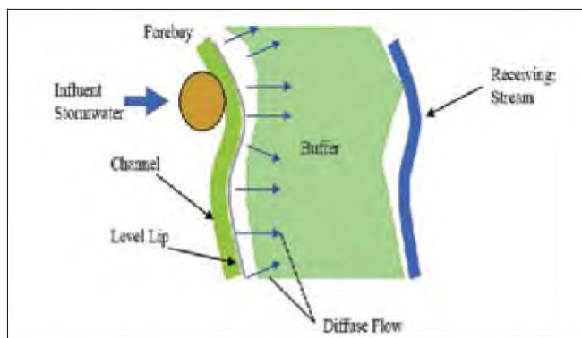
Level spreader located between a sediment forebay and a buffer
