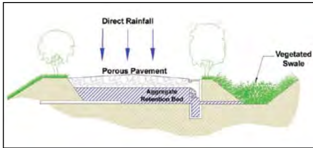
Figure 2: Slow discharge from porous pavement bed to vegetated swales Source: Pennsylvania Stormwater BMP Manual 2006
