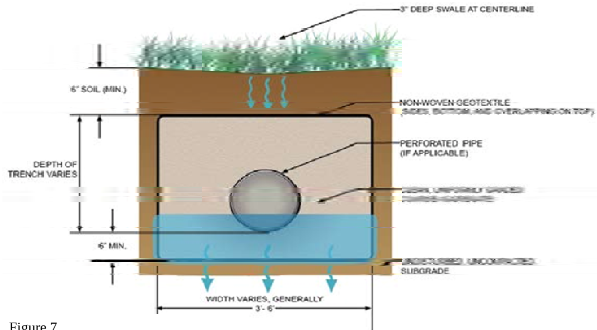
Figure 7 Infiltration trench cross section
