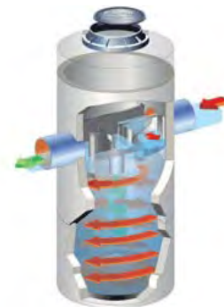
Plate Hydrodynamic Separator Source: Terre Hill Stormwater Solutions
