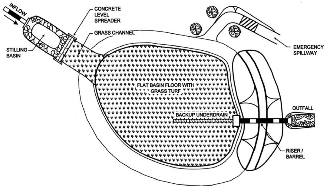
Figure 6. Infiltration Basin Sketch
