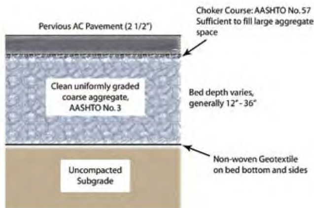
Figure 1: Example cross-section of porous asphalt system
