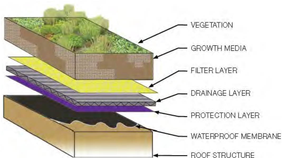
Figure 1 Single media assembly
