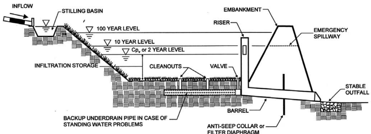
Figure 1: Residential Rain Garden with surface connection to subsurface infiltration bed under garden
