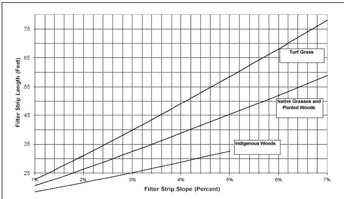
Figure 5: Sandy Soils with HSG Group A Source: New Jersey Stormwater Best Management Practices Manual, February 2004
