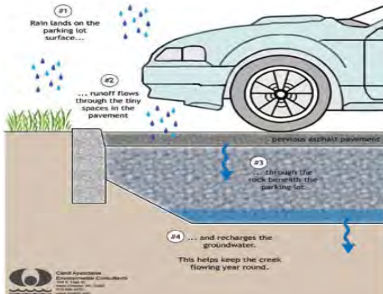
Pervious Pavement with infiltration schematic
