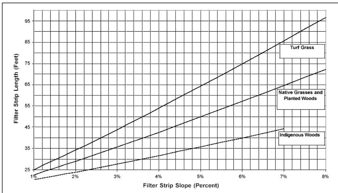
Figure 6: Sandy Loam Soils with HSG Group B Source: New Jersey Stormwater Best Management Practices Manual, February 2004
