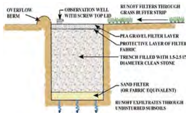
Filter with infiltration to subsoils
