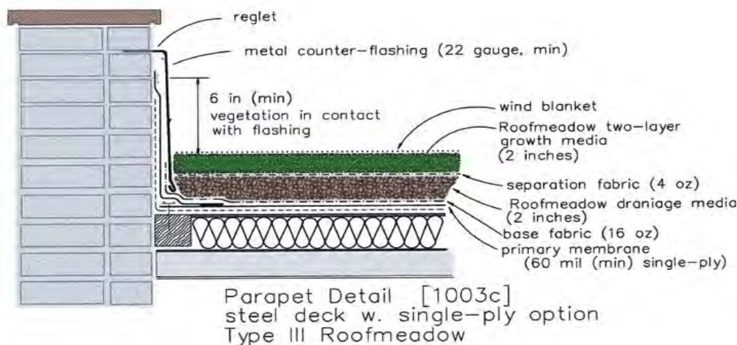
Figure 4: Example parapet flashing detail for flat roof Source: Roofscapes, Inc.
