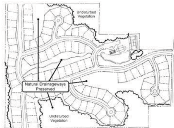
Schematic of a site design protecting natural drainage features. Source: Georgia Stormwater Management Manual, Volume 2: Technical Handbook, First Edition. August, 2001
