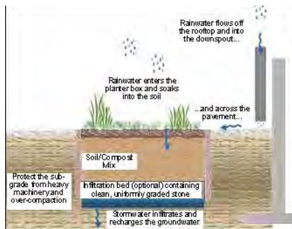
Figure 2 Schematic of Infiltration Planter Box
