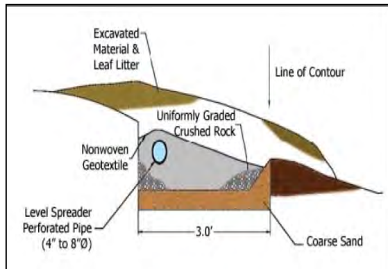
Level spreader with geotextile surrounding the aggregate helping to create a sloped area.
