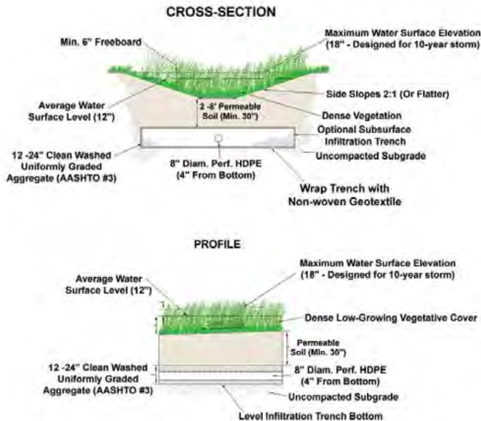
Figure 1: Schematics of Vegetated Swale with an underlying aggregate layer Source: Pennsylvania Stormwater BMP Manual, 2006
