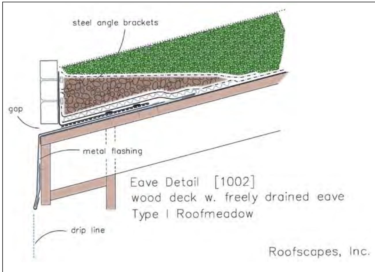
Figure 3: Example Eave Detail for sloped roofc.com Source: Roofscapes, Inc.
