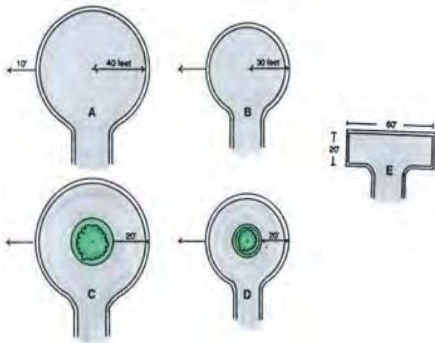
Figure 1: Five Cul-de-sac Options Source: Center for Watershed Protection, 1998
