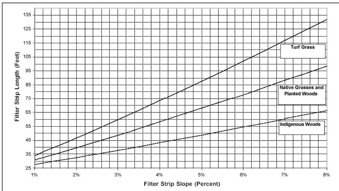
Figure 8: Sandy Clay Loam Soils with HSG Group C Source: New Jersey Stormwater Best Management Practices Manual, February 2004
