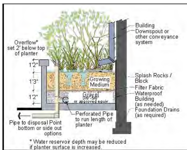
Figure 3 Schematic of Flow-through Planter Box
