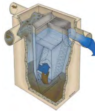
Vortex Hydrodynamic Separator Source: Stormwater Solutions
