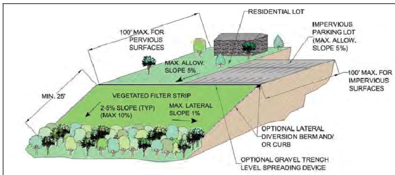
Figure 1 Diagram showing elements of a vegetated filter strip
