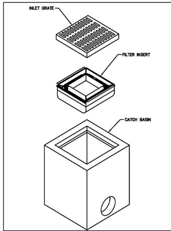
Figure 1: Tray Type Insert Source: Pennsylvania Stormwater BMP Manual, 2004
