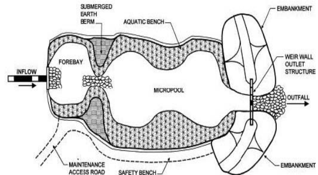
Figure 2: Pocket wet pond Source: Maryland Stormwater Manual, 2000
