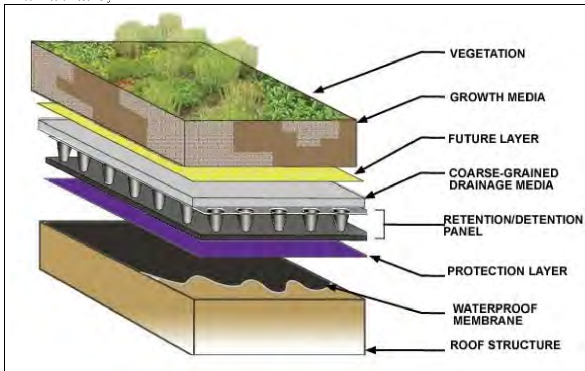
Figure 2 Dual Media Assembly
