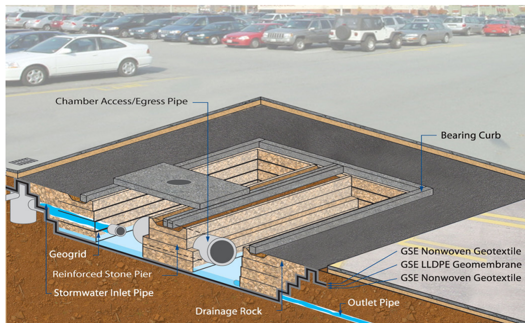
Schematic of underground detention facility, courtesy of CETCO Contracting Services
